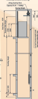
Hoistway Elevation Drawing
