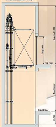
Hoistway Elevation Drawing
