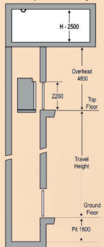
Hoistway Elevation Drawing
