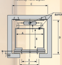
Hoistway Plane Layout
