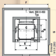
Hoistway Machine Room Plan For Manual Door
